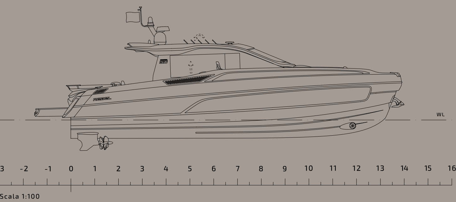
INBOARD PROFILE
