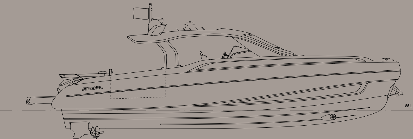
INBOARD PROFILE
